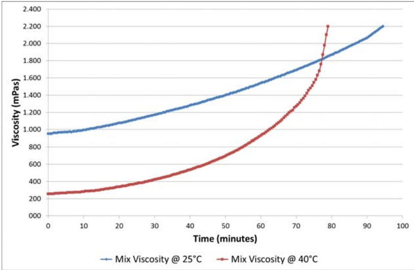
Graphic 1 – Mixed Viscosity of the System EC 180/W 340 at different temperatures
